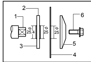
1. Mounting shaft 2. Inner flange 3. 25.4 mm marking 4. Diamond wheel 5. Outer flange 6. Hex bolt
