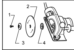
1. Hex bolt 2. Diamond wheel 3. Outer flange 4. Inner flange
